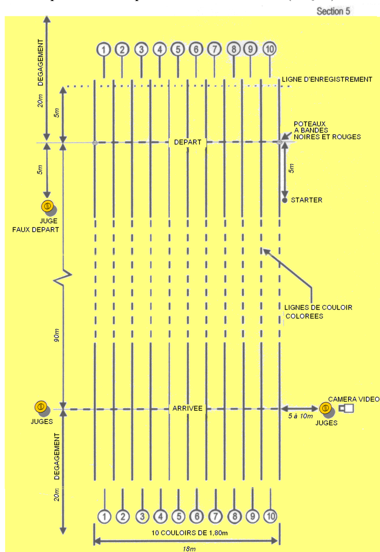
RELAIS SPRINT
